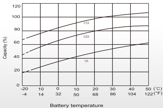
Effects of Temperature on Capacity
