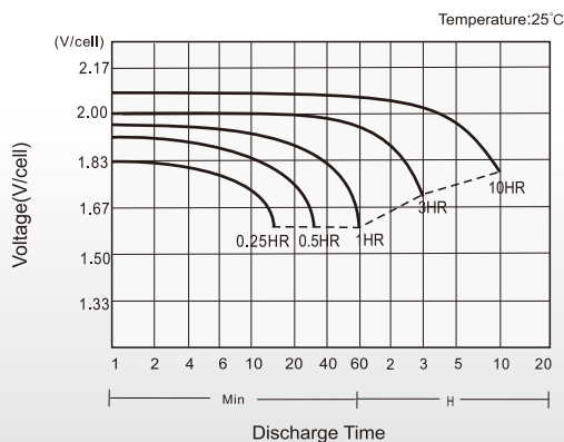
Discharge Characteristics
