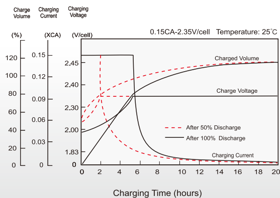
Charging Characteristics
