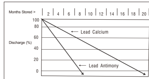
Figure 2 Self Discharge Rate Calcium Vs. Antimony @ 77°F
